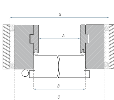
Dimensions of the 42dB fixed MDF door frame [mm]
