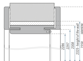
▼ Dimensions of the door frame for the Natura HK PN23 door.
