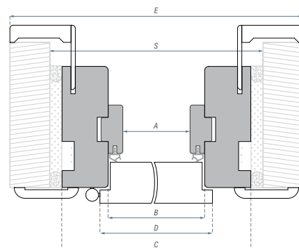
Dimensions of the BORD MDF door frame [mm]:
