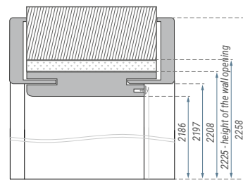
▼ Dimensions of the door frame for the Natura HB PN22 door.
