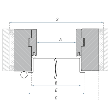
Dimensions of fire-rated wooden fixed and adjustable door frame [mm]
