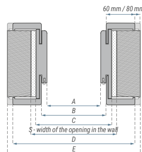
▼ Dimensions of the door frame for the Natura HK PN22 door.
