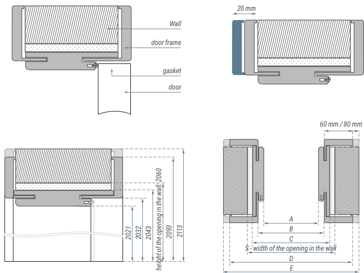
▼ Dimensions of the door frame for the Natura HB PN21 door.
