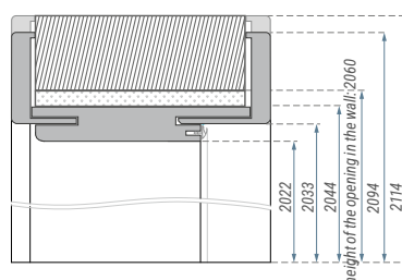
▼ Dimensions of the door frame for the Natura HK PN21 door.
