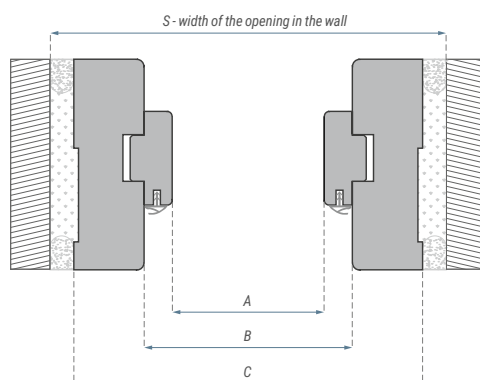
Standard 2-pack door frame dimensions [mm]:
