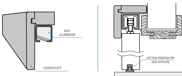
VERTICAL CROSS-SECTION OF THE SLIDING SYSTEM
