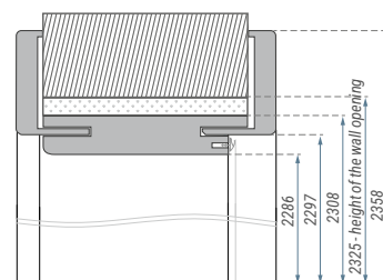
▼ Dimensions of the door frame for the Natura HB PN23 door.
