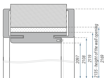
▼ Dimensions of the door frame for the Natura HK PN21 door.
