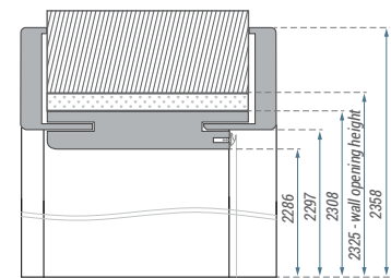
▼ Dimensions of door frame for Natura HK PN23 door.
