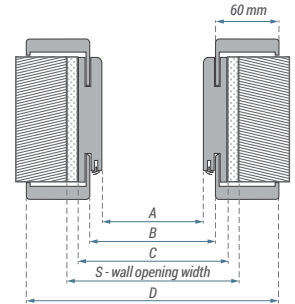
▼ Dimensions of door frame for Natura HK PN23 door.
