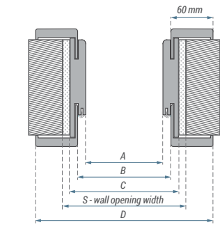
▼ Dimensions of door frame for Natura HB PN23 door.
