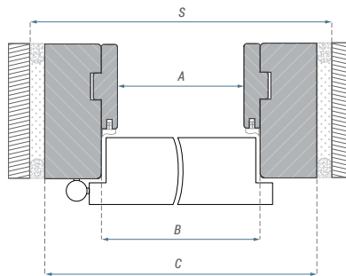
Dimensions of 42dB MDF fixed door frame [mm]:
