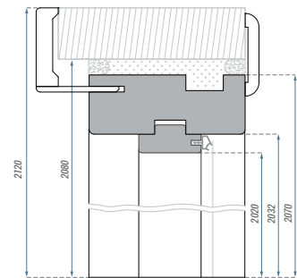
BORD ADJUSTABLE MDF ▼
