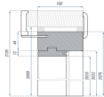
42 DB MDF ADJUSTABLE ▼
