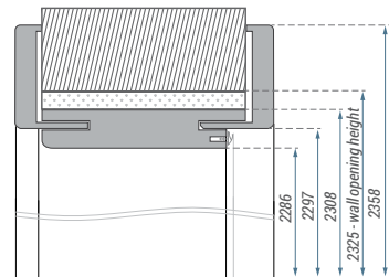
▼ Dimensions of door frame for Natura HB PN23 door.
