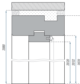
BORD MDF FIXED ▼
