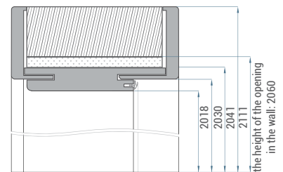
▼ Non-rebated adjustable door frames 80
