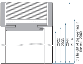
Dimensions of the adjustable door frame [mm]:
