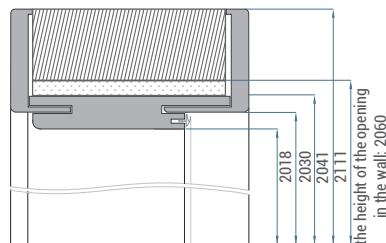
Dimensions of the adjustable non-rebated door frame [mm]:
